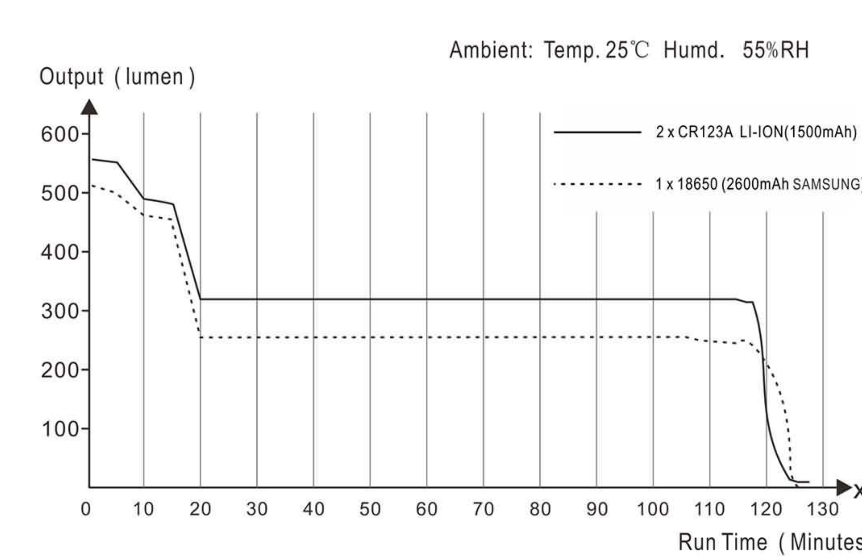
Figure 4 Output VS Runtime/运行曲线
