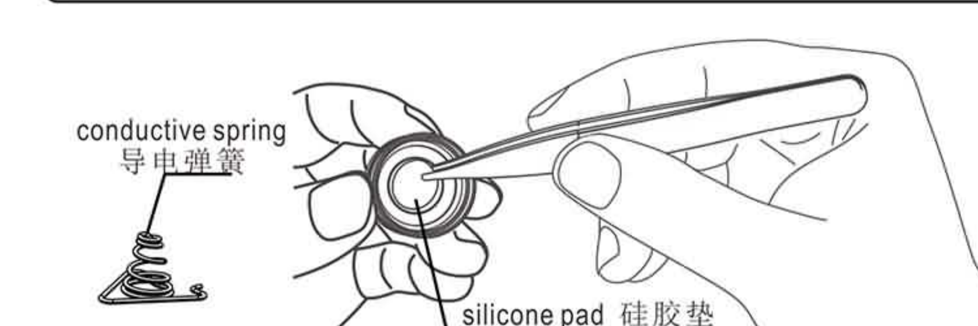
Figure 5 How to remove the magnet of S20-L2 Baton/如何替换S20-L2 Baton尾盖的磁铁
