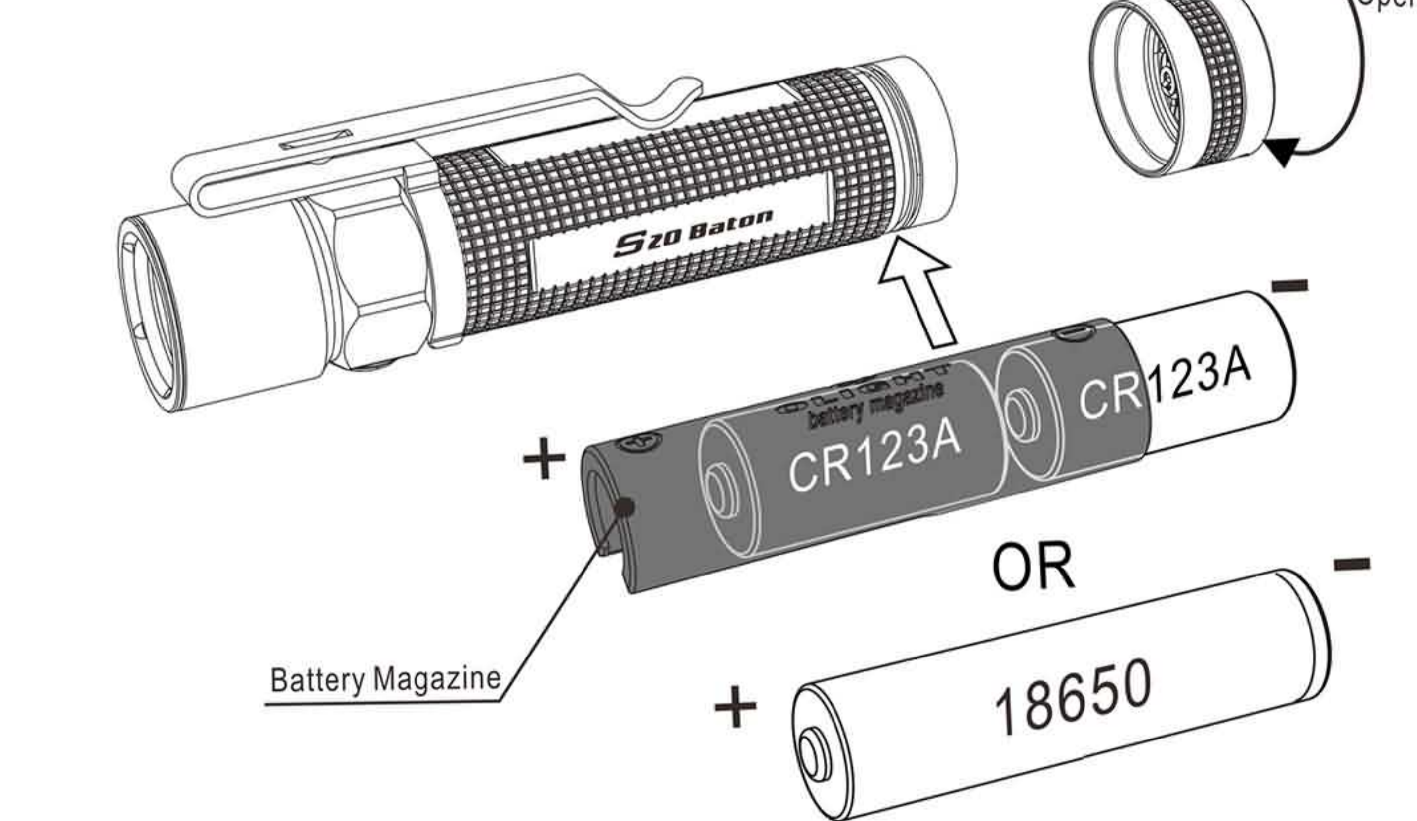
Figure 2 Battery installation/电池安装
