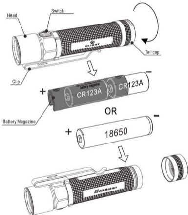
Figure 1 Product parts & Battery installation 产品部件与电池安装
