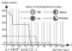
Figure 3 Output VS Runtime 运行曲线
